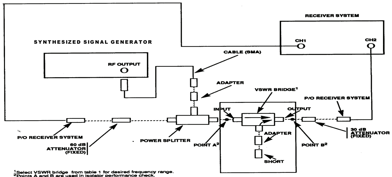
Figure 1. VSWR, insertion loss and isolation equipment setup.
